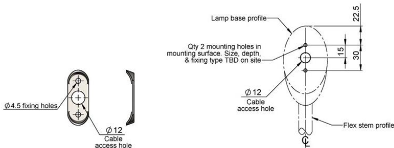
MOUNTING BRACKET Dimensions in mm
