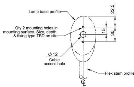
RECOMMENDED MOUNTING HOLE DETAILS Dimensions in mm
