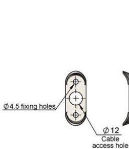
MOUNTING BRACKET Dimensions in mm
