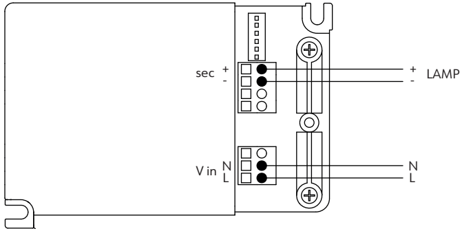
PUSH wiring diagram
