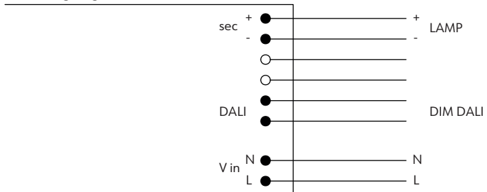
DALI wiring diagram
