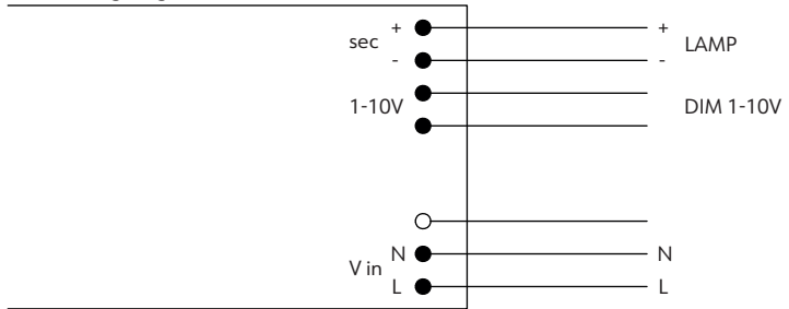
1-10V wiring diagram
