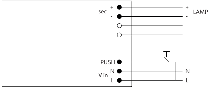
PUSH wiring diagram
